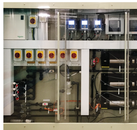
800 m³/h (3500 gpm) NITRASEP® Plant
